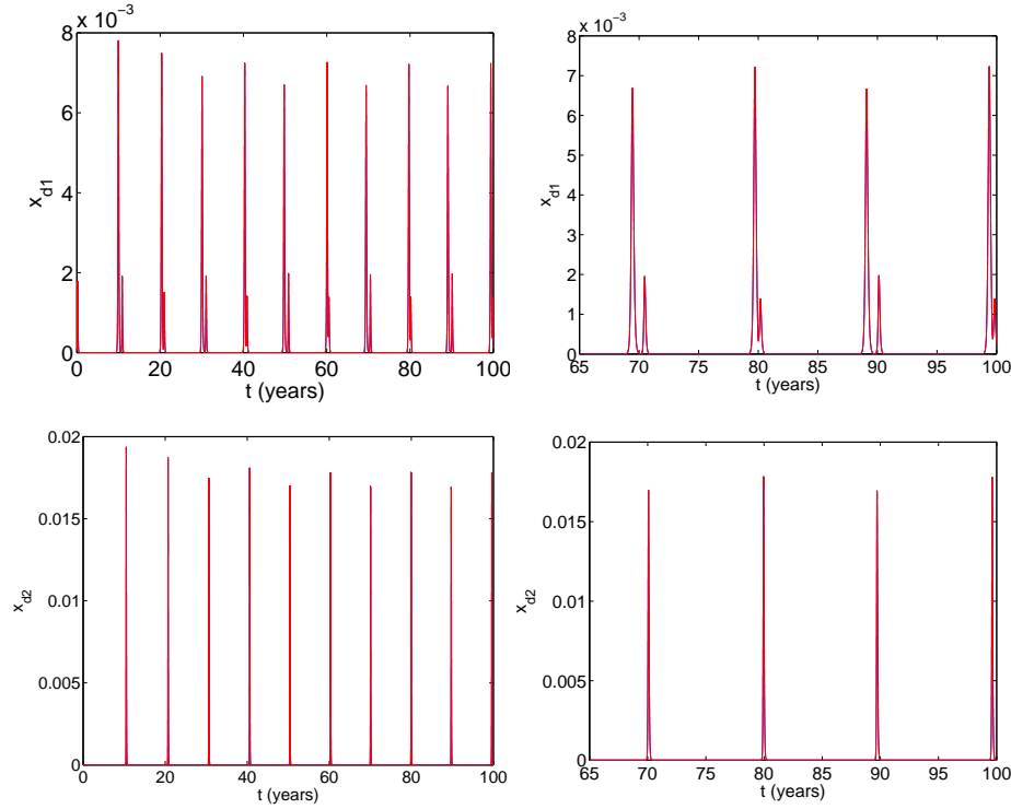
Fig. 3 Plots of (a)-(b) x_{d1} and (c)-(d) x_{d2} computed using the complete system of equations (blue) and the center manifold equation (red) for (a) and (c) t = 0 to t = 100 , and (b) and (d) t = 65 to t = 100 . Parameter values are given by \mu = 0.02 , \sigma = 50.0 , \phi = 3.0 , and \beta = 200.0 .
