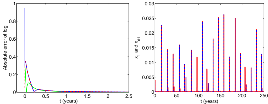
Fig. 5 (a) Absolute error in log variables for susceptibles and primary infectives versus time. Solid green: |\log s_d - \log s| , solid blue: |\log x_{1d} - \log x_1| , dashed red: |\log x_{2d} - \log x_2| . The initial condition for the driver system was a point on the chaotic attractor obtained by computing a long time series. The initial condition for the driven system was a random perturbation with mean 10% away from the driver system. (b) Time series showing synchronization of x_1 (solid red) and x_{d1} (dashed blue). Parameter values are the same as in Fig. 4.
