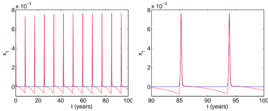
Fig. 2 Plot of x_1 computed using the complete system of equations (blue) and the center manifold equation (red) for (a) t = 0 to t = 100 , and (b) t = 80 to t = 100 . Parameter values are given by \mu = 0.02 , \sigma = 50.0 , \phi = 3.0 , and \beta = 200.0 .
